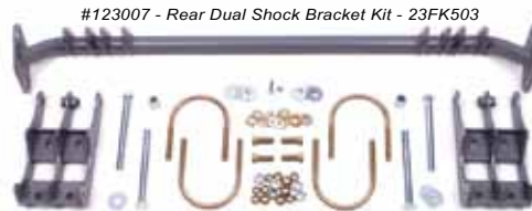
#123007 - Rear Dual Shock Bracket Kit - 23FK503 Note: Will not fit dually equipped vehicles or Excursion
